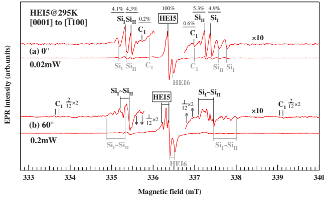
FIG. 2. (Color online) Hyperfine structures of HEI5 center in 4H-SiC. (a) 0^\circ spectrum of HEI5 measured during magnetic-field rotation from [0001] ( 0^\circ ) to [\bar{1}100] ( 90^\circ ) using microwave of 0.02 mW (9.428 GHz). In this condition, both HEI5 and HEI6 signals were detected at the same time without microwave saturation behavior. We give intensity ratio of each HF satellite line to a central line for HEI5, supposing that overlapped HEI6's HF lines have their ideal intensities (9.4% for \text{Si}_I and 0.55% for \text{C}_1 ). (b) 60^\circ spectrum of HEI5. \text{C}_1 HF structure of HEI5 splits into eight satellite lines with intensity ratio of 2:2:1:1:1:1:2:2 [see an angular map in Fig. 4(b)], and outer four lines can be resolved. Asterisks (*) indicate positions of missing ^{13}\text{C} satellite lines of HEI5.
