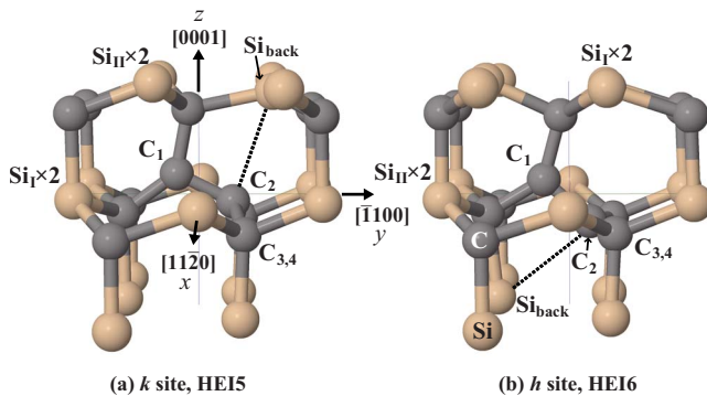
FIG. 5. (Color online) Atomic structures of dicarbon antisites or HEI5/6 centers at k and h sites in 4H -SiC. They have a single negative charge ( S=1/2 ) and C_{1h} symmetry with respect to the (11\bar{2}0) plane ( yz plane). These figures reproduce the atomic positions obtained from the first-principles calculation. The Cartesian coordinate system is also shown in the figure. Note the opposite locations of Si_I and Si_{II} atoms with respect to the C_1 and C_2 atoms between (a) and (b). The dashed line represents the weak interaction between the C_2 atom and a third-neighbor Si atom labeled Si_{back} .
