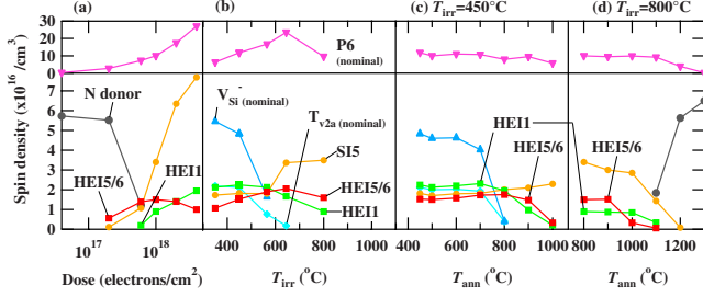
FIG. 6. (Color online) Formation and annihilation of HEI5/6 and other coexisting centers in n -type 4 H -SiC. Panels (a) and (d) are replotted from Ref. 6. (a) Electron dose was varied (zero, 2 \times 10^{17} to 4 \times 10^{18} e/cm^2 ) for six n -type 4 H -SiC substrates kept at T_{irr}=800 °C. (b) The same dose ( 1 \times 10^{18} e/cm^2 ) was applied and the irradiation temperature ( T_{irr} ) was varied for five n -type 4 H -SiC substrates. (c) and (d) Isochronal annealing measurements for samples of T_{irr}=450 and 800 °C, respectively. Spin densities of N(k) donors and HEI5/6 were estimated in the dark at 70 K, while those of SI5 and HEI1 were estimated under photoillumination (100 W halogen light) because these centers were stabilized in EPR-inactive states in the dark. Those of P6 and V_{Si}^-/T_{V2a} are nominal values (respectively, estimated at 30 and 295 K under photoillumination) because they have a triplet ( S=1 ) or a quartet spin ( S=3/2 ) and their EPR signals are enhanced by optically induced spin polarization.
