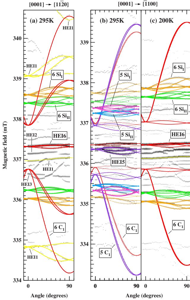
FIG. 4. (Color online) Angular maps for HEI5/6 centers ( ^{13}\text{C} and ^{29}\text{Si} hyperfine satellite lines). \mathbf{B} was rotated either in the (\bar{1}100) plane ( [0001] \rightarrow [11\bar{2}0] ) or in the (11\bar{2}0) plane ( [0001] \rightarrow [\bar{1}100] ). “+” symbols present resonant positions (larger and darker symbols indicate larger resonant peaks). Solid lines were calculated by using the spin-Hamiltonian parameters shown in Tables I and II or by using those in Ref. 4 (for HEI1). “C 1 ” indicates the ^{13}\text{C} hyperfine interaction due to a carbon interstitial atom in HEI5/6. “Si I ” and “Si II ” denote ^{29}\text{Si} hyperfine interactions from four Si atoms surrounding an interstitial atom (see details in the text). (a) Angular pattern for HEI6 at 295 K. This map was produced using a series of HEI6 spectra shown in Figs. 1(b) and 1(c). (b) Angular patterns for a combination of HEI5 and HEI6 at 295 K. This map was produced using a series of EPR spectra shown in Fig. 2(b). Four inner branches of C 1 were not resolved due to their small intensities and interferences from many small signals over a middle region [cf. Fig. 2(b)]. Note that the HEI5’s pattern was temperature independent, but the HEI6’s pattern was temperature dependent above 150 K. (c) Angular pattern of HEI6 at 200 K. This map was produced using a series of HEI6 spectra shown in Fig. 1(d). Four inner branches of C 1 could not be resolved again. Also some branches of Si I and Si II were unclear in the map due to overlaps between the satellite lines [cf., Fig. 1(d)]. At this temperature, HEI1/2 signals became larger and disturbed observation of some central lines of HEI6 [cf., Fig. 1(d)].
