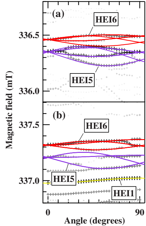
FIG. 3. (Color online) Angular maps of HEI5/6 centers (primary lines). The magnetic field was rotated by 90^\circ in the following directions: (a) [\bar{1}100] and (b) [0001] \rightarrow [11\bar{2}0] . Solid lines show simulated angular patterns. EPR measurements were carried out under the same conditions as in the measurements of Fig. 1(a). These maps were measured using different microwave frequencies.
